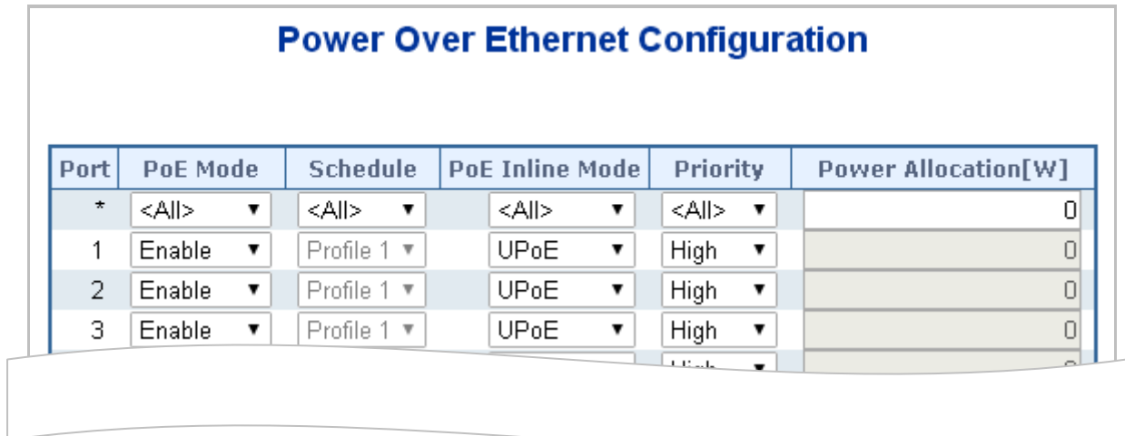
Figure 4-16-4: Power over Ethernet Configuration Screenshot
