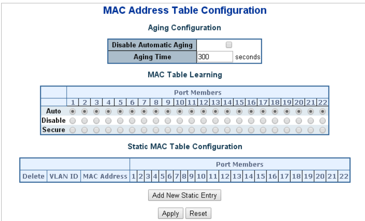
Figure 4-13-1: MAC Address Table Configuration Page Screenshot
