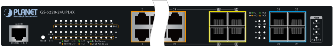
Figure 2-1-21: GS-5220-24UPL4X LED on Front Panel
