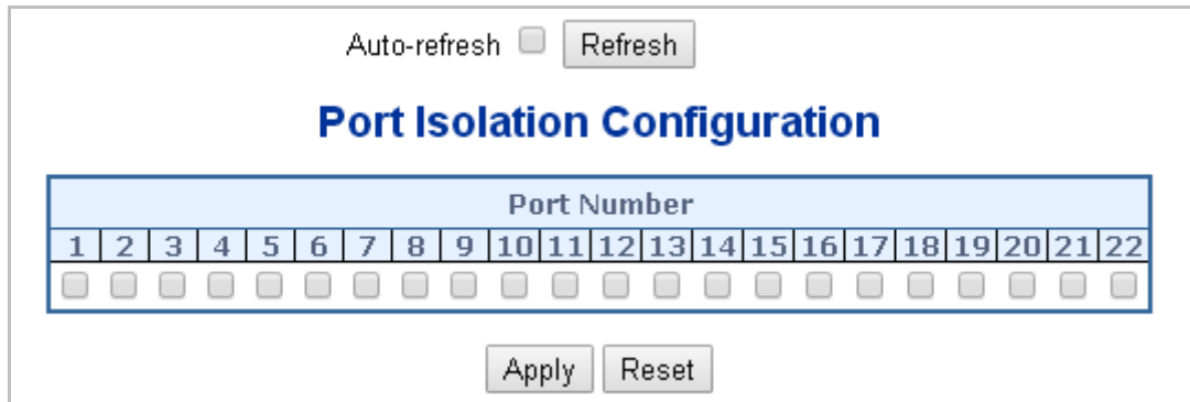
Figure 4-6-6: Port Isolation Configuration Page Screenshot
