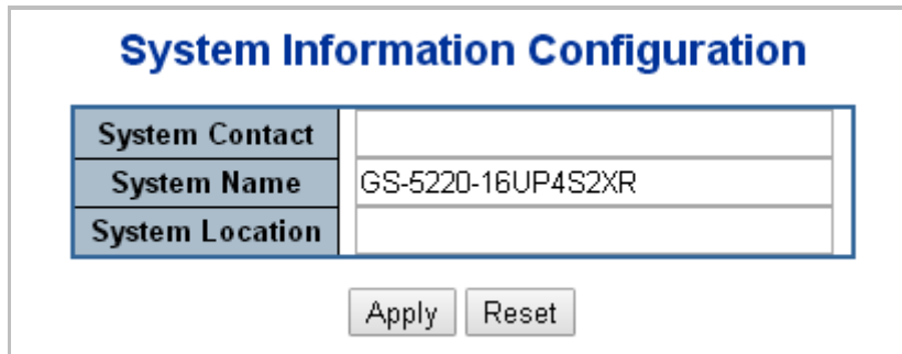
Figure 4-3-3: System Information Configuration Page Screenshot
