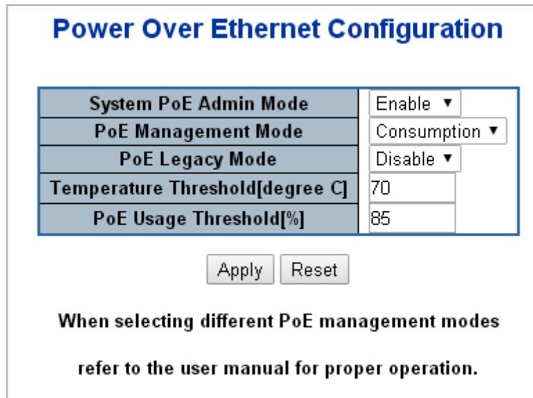
Figure 4-16-2: PoE Configuration Screenshot
